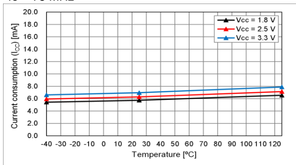
fo = 75 MHz
