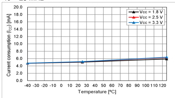
fo = 25 MHz
