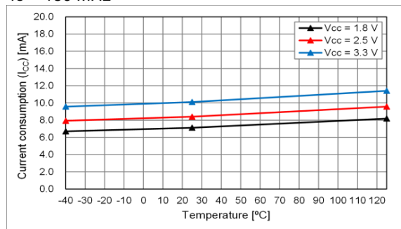
fo = 150 MHz
