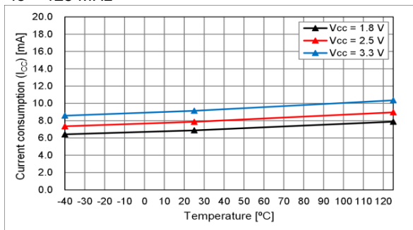
fo = 125 MHz
