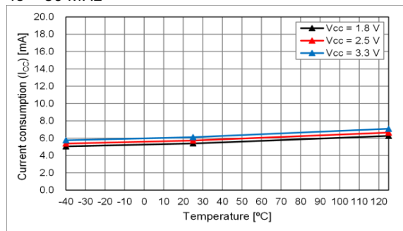
fo = 50 MHz
