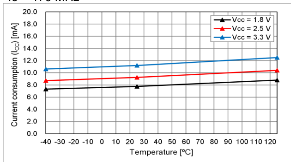
fo = 170 MHz
