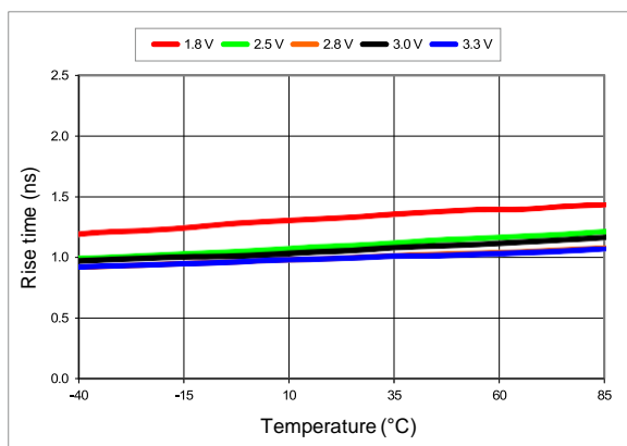
Figure 12. 20%-80% Rise Times vs Temperature
