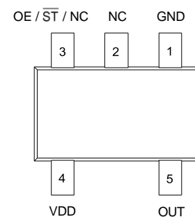
Figure 1. Pin Assignments
