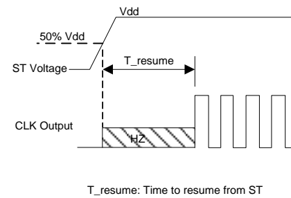
Figure 6. Standby Resume Timing ( \overline{\text{ST}} Mode Only)
