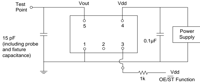
Figure 2. Test Circuit [6]
