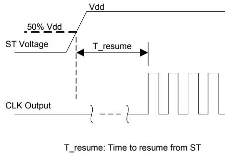
Figure 8. Standby Resume Timing ( \overline{ST} Mode Only)
