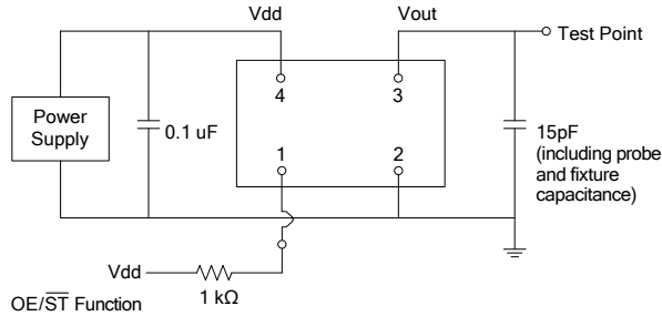
Figure 2. Test Circuit
