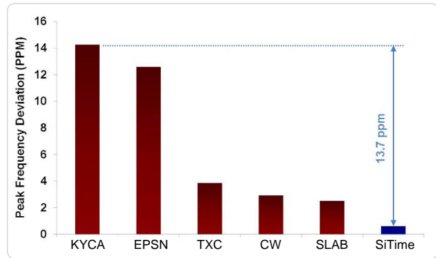
Figure 20. Shock Robustness [6]
