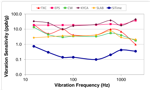
Figure 19. Vibration Robustness [5]
