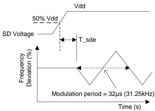
Figure 6. SD Enable Timing (SD Mode Only)
