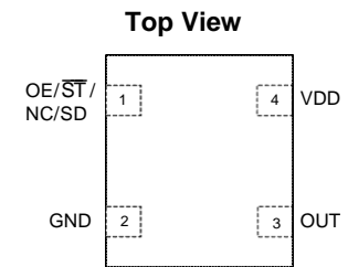
Figure 1. Pin Assignments
