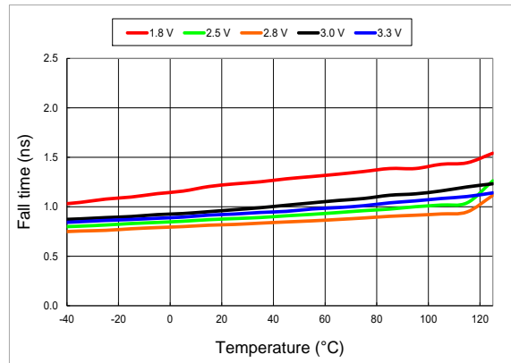
Figure 10. 20%-80% Fall Time vs Temperature
