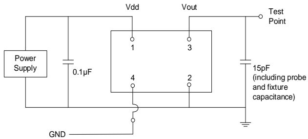
Figure 2. Test Circuit [8]
