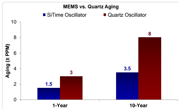
Figure 2. Aging Comparison [2]
