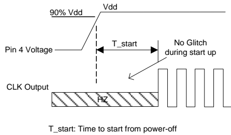
Figure 4. Startup Timing [11]
