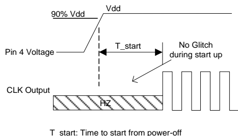
Figure 4. Startup Timing [11]
