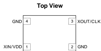
Figure 1. Pin Assignments
