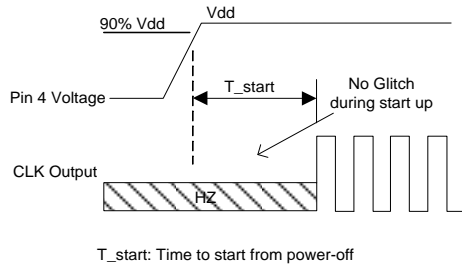
Figure 4. Startup Timing [11]
