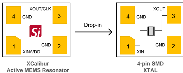
Figure 20. XCalibur Active MEMS Resonator compared with 4-Pin SMD XTAL (TOP View)
