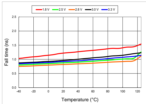
Figure 10. 20%-80% Fall Time vs Temperature
