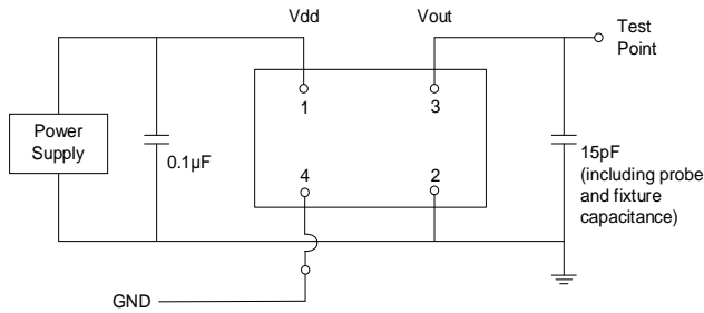
Figure 2. Test Circuit [10]
