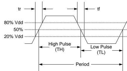
Figure 3. Waveform [10]
