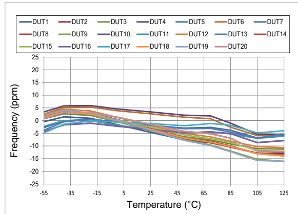
Figure 6. Frequency vs Temperature
