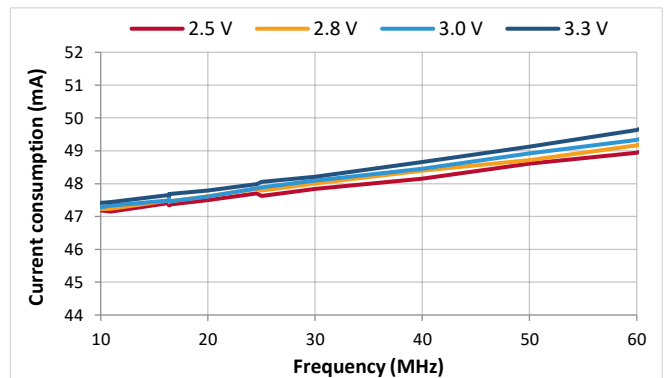
Figure 33. IDD VTCXO (LVCMOS)
