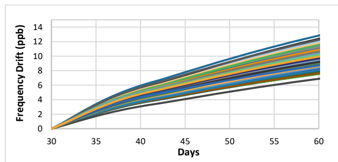
Figure 27. Frequency drift after 30 days [16]
