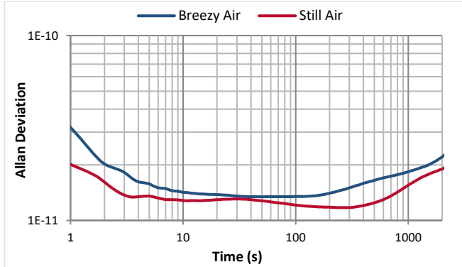
Figure 20. ADEV [15]
