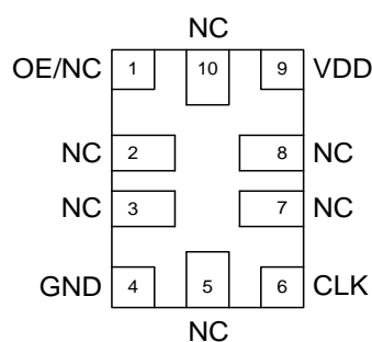
Figure 3. TCXO
