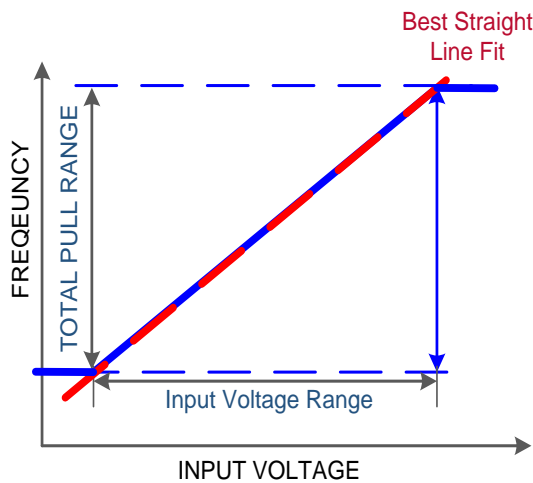
Figure 49. Typical SiTime VCTCXO Linearity
